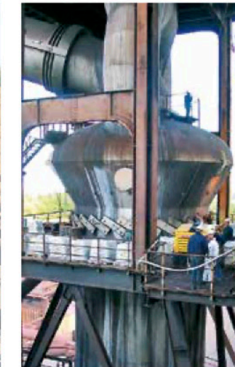
Short lining times for a whirler are achieved with a combined lining of hard compound KALCRET BTS and zirconium corundum KALCOR. The high application rate of KALCRET BTS is 5 m 2 /h
